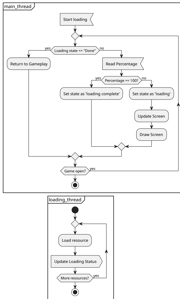
Figure 390: Rough UML diagram of a multi-threaded loading screen
